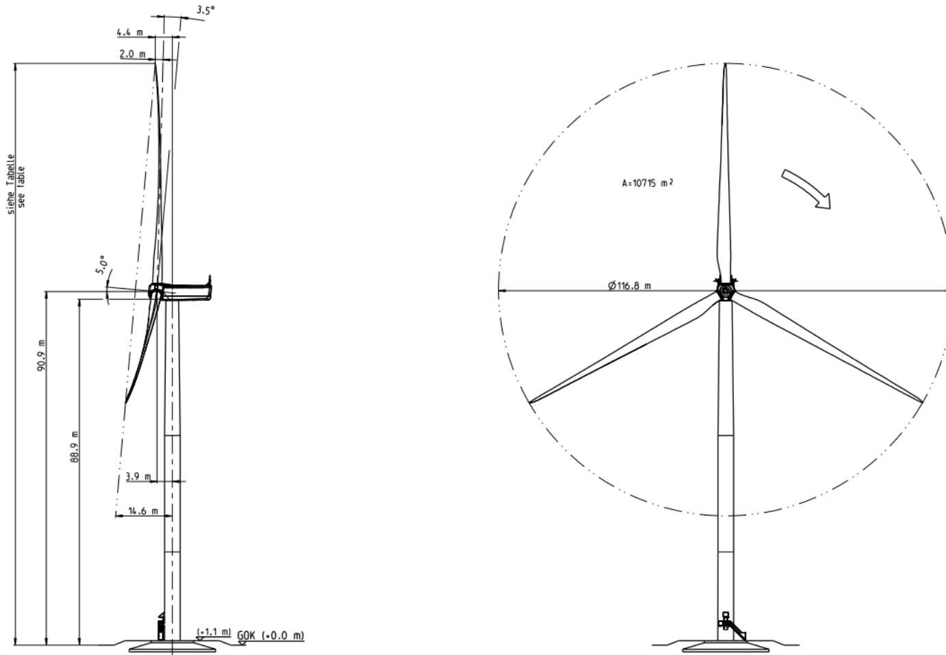
FIGURE 15 : NORDEX – N117 (2/2)
