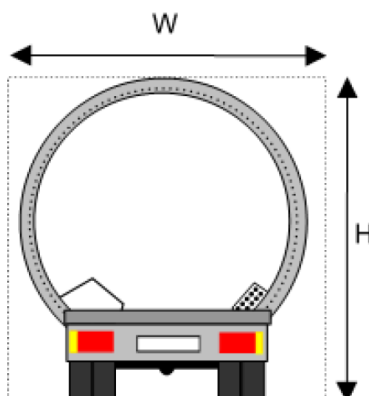
FIGURE 17 : COUPE PROFIL VEHICULE TRANSPORT EOLIENNE (H = 5 M / W = 5 M)
